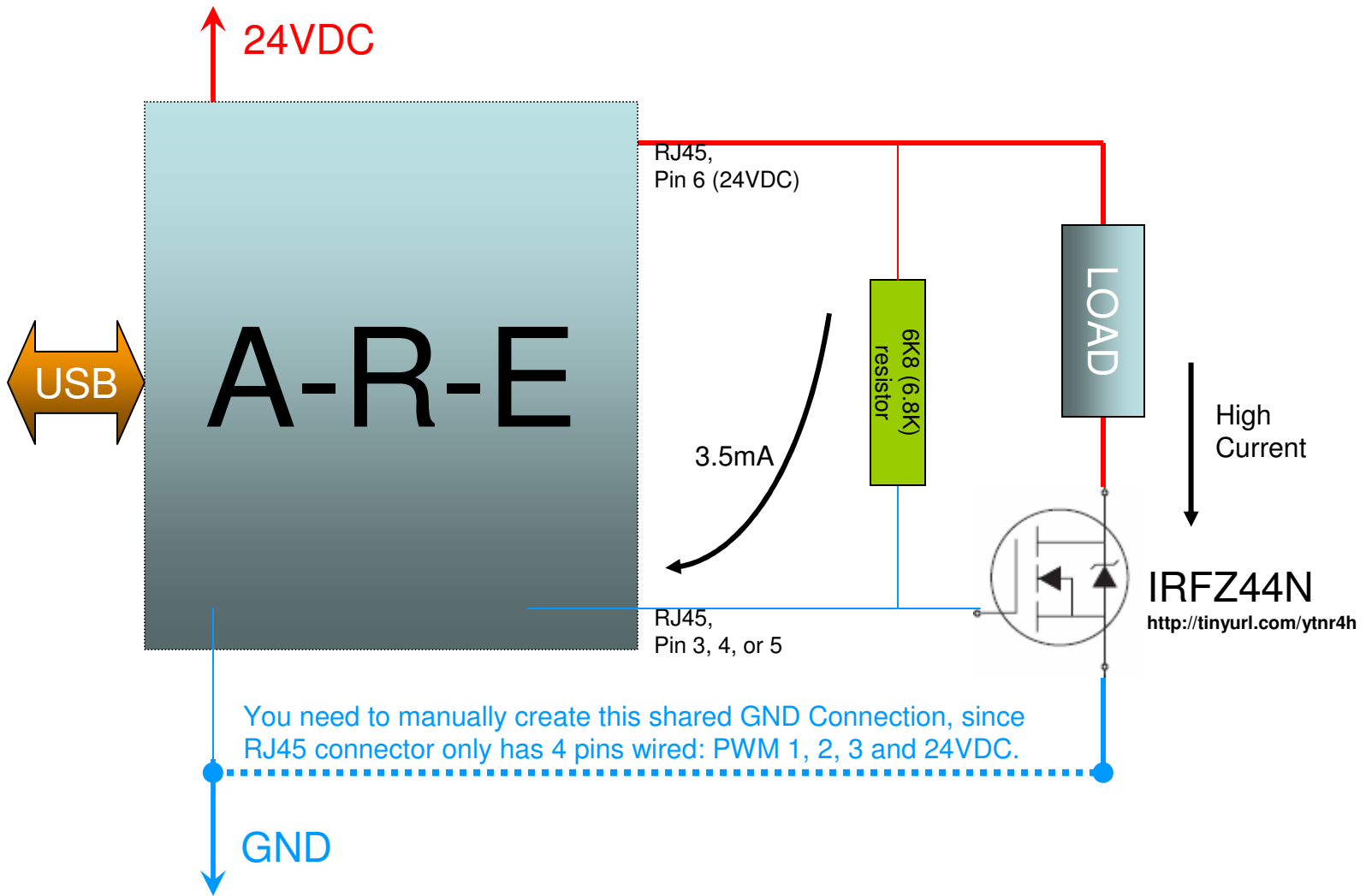
High Current Loads - MOSFET
