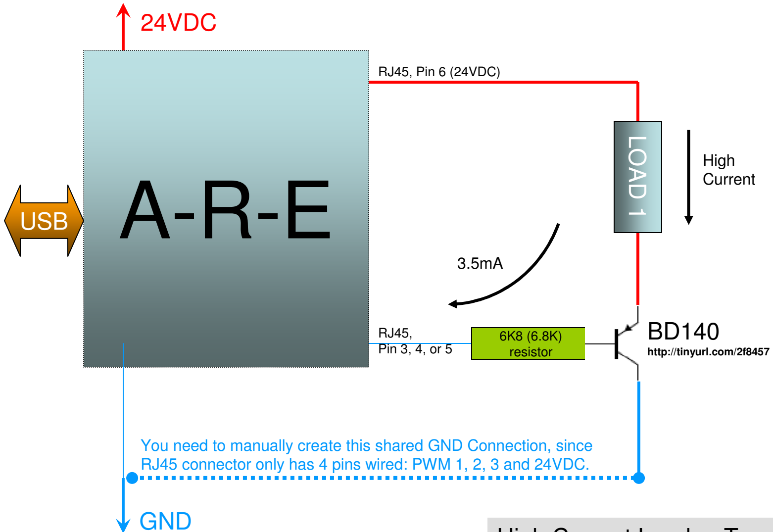
High Current Loads - Transistor
